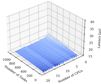
(c) RR/FP Plugin
