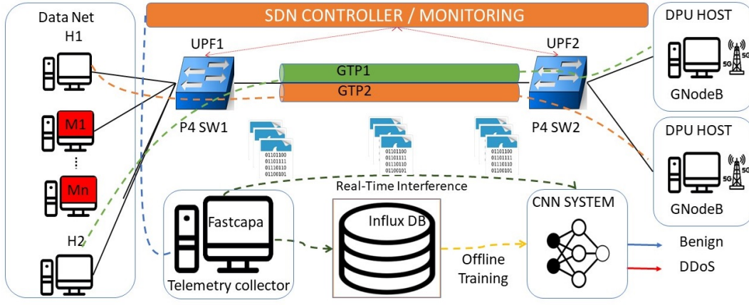
Fig. 1: Proposed Framework Network Topology
