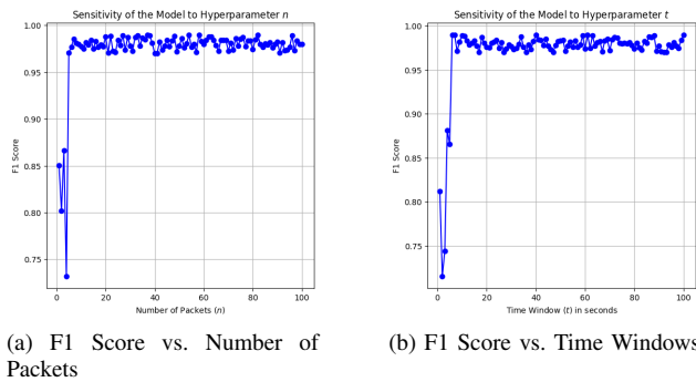
Fig. 3: The model's sensitivity to the hyperparameter n for F1 score.
