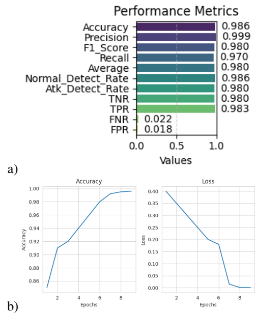
Fig. 4: Performance Metrics and Loss: a) Performance metrics of the CNN model for DDoS attack detection. b) Accuracy and loss of the CNN model throughout training on P4 telemetry data.
