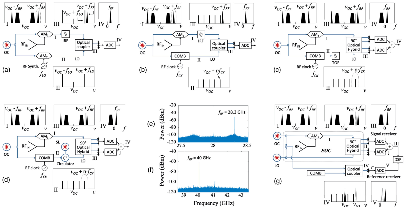
Fig. 2. (a)–(d), (g) MWP coherent architectures. Insets depict optical or RF signals at different points. (e), (f) Power spectrum of the noise-free reconstructed SUT, produced by the injection-locking-based receiver of scheme (d) [31], and the FF receiver with SiP modulator of scheme (g) [32], respectively, when 28.3 and 40 GHz tones are used as input. OC, optical carrier; LO, local oscillator; AM, amplitude modulator; IRF, image-reject filter; TOF, tunable optical filter; EOC, electro-optic converter.
