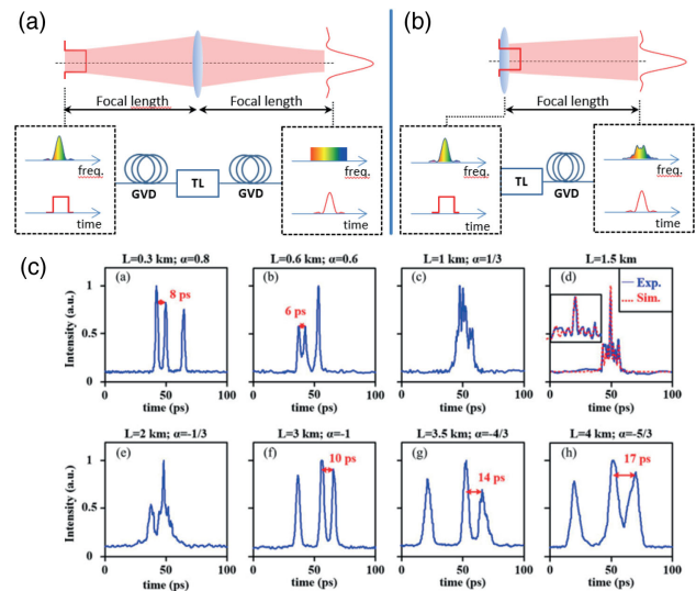
Fig. 4. (a) Fourier analysis by means of the 2f setup in the space (top) and time (bottom) domains. GVD and TL are respectively equivalent to free-space propagation and a thin lens. (b) Simplified setup for Fourier analysis, where the first dispersion step is omitted [71]. (c) Example of spectral analysis of a digital RF input signal modulated on an optical carrier based on the combination of an electro-optic TL and a dispersive fiber. The blue traces represent the intensity of the waveform along the fiber. At the proper propagation distance ( L = 1.5 km), the intensity maps the spectrum of the RF SUT. Reprinted with permission from [72] © The Optical Society.
