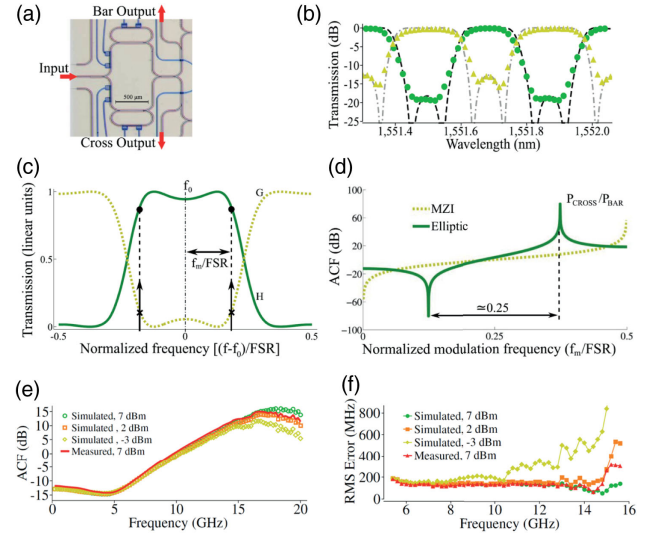
Fig. 7. Photonic IFM system based on a RAMZI filter. (a) Microscope photograph of the filter. (b) Simulated and measured bar (circles) and cross (triangles) responses. (c) Operation principle; (d) simulated and (e) measured ACF; (f) root-mean-square error. Adapted with permission from [119] © The Optical Society.
