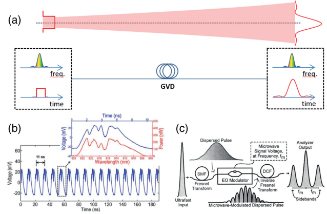
Fig. 3. Space–time duality and D-FTM. (a) Equivalence between the diffraction in the far field of an input spatial wavefront and the propagation of an input temporal waveform through GVD, leading to D-FTM. (b) Example of D-FTM: the temporal waveform of a pulse recorded by an oscilloscope precisely maps the pulse spectrum measured by a conventional optical spectrum analyzer. Reproduced under the terms of the CC-BY Creative Commons Attribution 4.0 International License [52]. Copyright 2012, Macmillan Publishers Limited (now Springer Nature). (c) Principle of Fourier analysis of RF signals by combining the modulation of a chirped light pulse, with dispersive propagation. Reprinted with permission from [53] © The Optical Society.
