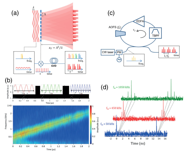
Fig. 5. Fourier analysis through periodic sampling. (a) A periodic waveform (wavelength \lambda ) is sampled by a transmission grating. For specific propagation distances (e.g., the Talbot length z_T ), the intensity maps repeatedly the input angular spectrum. In the time domain, the process is equivalent to sampling followed by GVD. (b) Demonstration of real-time spectrogram analysis by temporal sampling and GVD (bottom plot, showing the evolution of the time-mapped spectrum, vertical axis, along the time domain, horizontal axis) of an input linearly chirped microwave signal (top plot) [87]. (c) Fourier analysis based on FSL: the interference of replicas of the SUT, simultaneously shifted in both time and frequency, results in a time trace mapping the input signal frequency spectrum. (d) Example of high-resolution FTM in a FSL for input microwave tones of different frequency values, f_m . Adapted with permission from [88] © The Optical Society.
