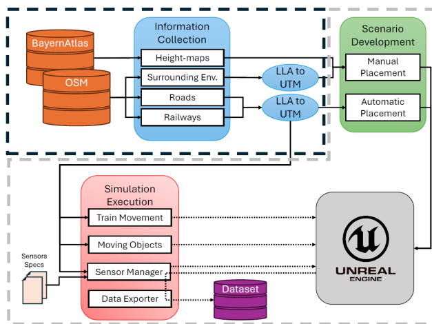
Figure 2. Block diagram of the dataset generation process.
