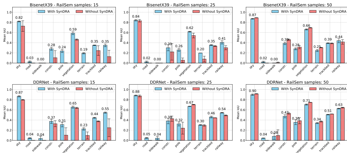
Figure 6. Finetuning results for Bisenet (top) and DDRNet (bottom) using different amounts of RailSem samples (15, 25, 50) with (blue) and without (red) SynDRA samples. The tests were conducted over 3 runs, with the variation shown by error bars. In these runs, the selection of samples from SynDRA and RailSem, as well as the seeds for applying data augmentation transformations, were randomized.
