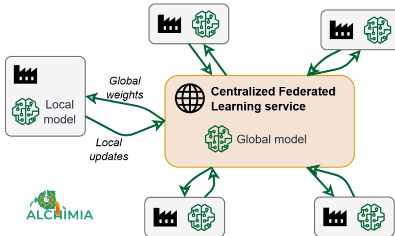
Figure 3. In Federated Learning, the global model enables the local models to be improved
