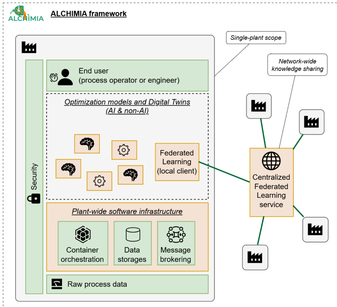
Figure 2. ALCHIMIA framework from the viewpoint of a production plant
