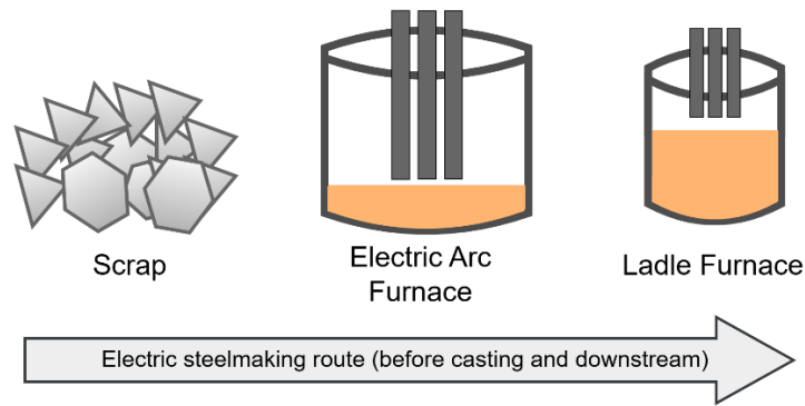
Figure 1. Electric steelmaking route
