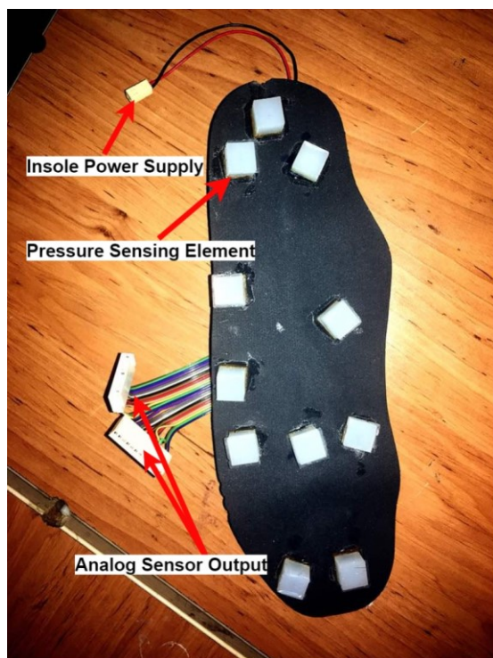
Fig. 10. Insole of ShrewdShoe ready to be placed inside the shoe. It's worth mentioning that another thin layer of fabric will eventually come on top to hide the sensors.
