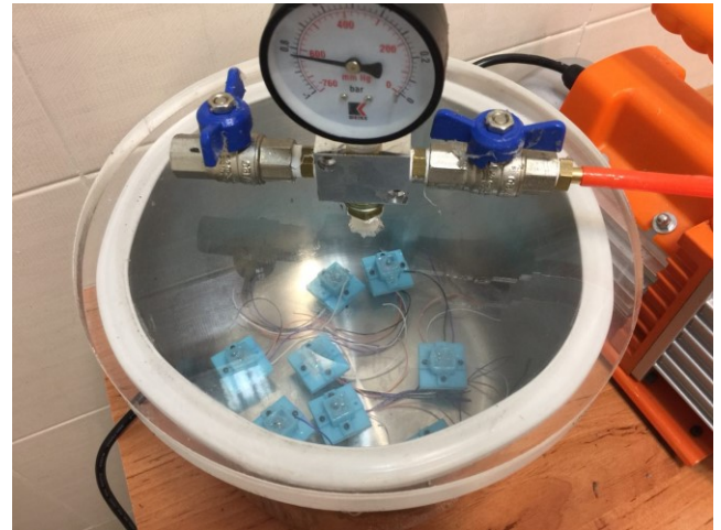
Fig. 8. The vacuum chamber used for degassing the silicon.
