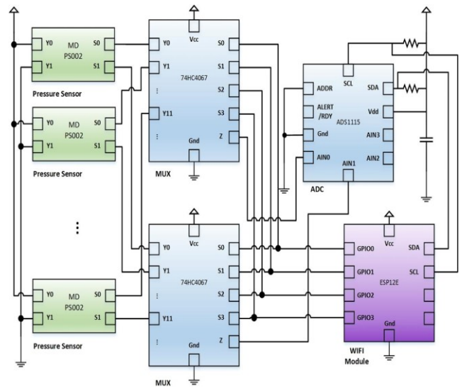
Fig. 4. Hardware schematic, consisting of an IoT module, an ADC module, two 16-to-1 multiplexers, and eleven sensors.
