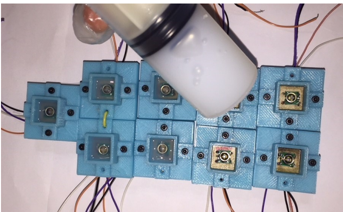
Fig. 7. Injection of RTV silicon into the molds.
