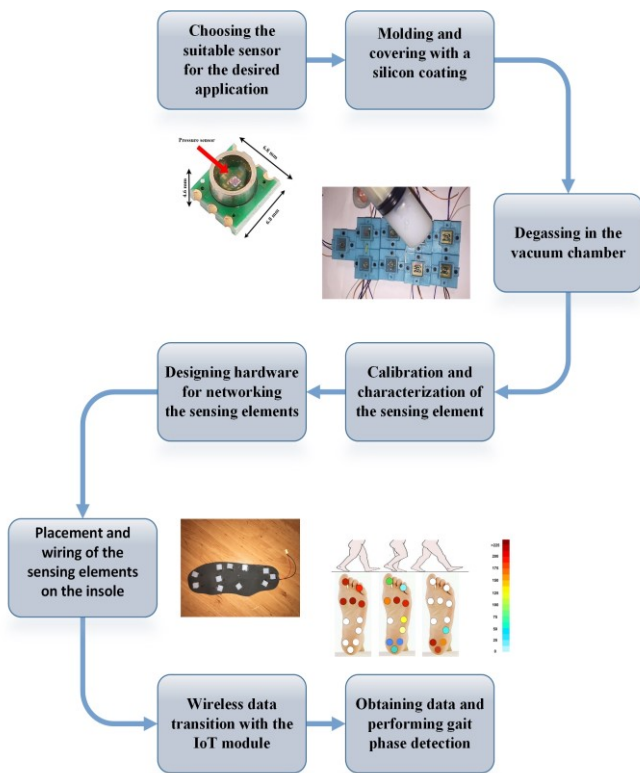
Fig. 1. This flowchart briefly demonstrates the design and development procedure of ShrewdShoe.
