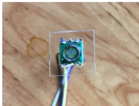
Fig. 5. Barometric sensor mounted on a plexiglass base.
