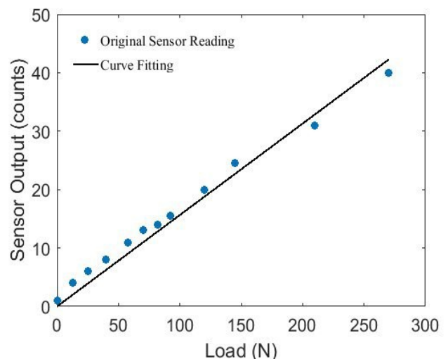
Fig. 9. This chart was plotted with MATLAB curve fitting tool for the data obtained from one of the sensing elements. This shows the promising linearity of our sensing element for ranges up to 300 N.
