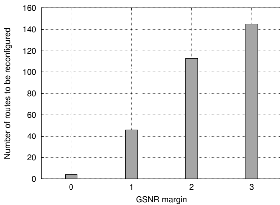
Fig. 8. Number of routes requiring reconfiguration when exploiting S-band versus margin M
