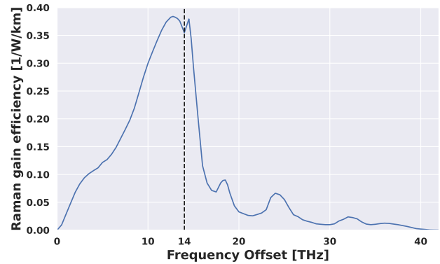
Fig. 3. Raman gain efficiency versus frequency offset for a SSMF.
