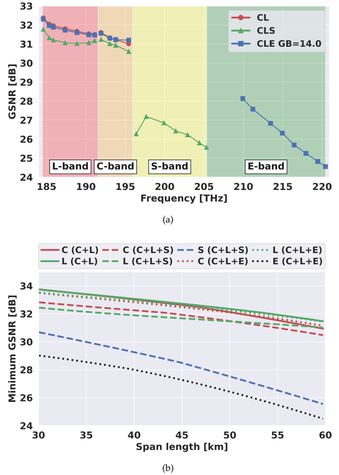
Fig. 5. (a) GSNR profile versus frequency for C+L-, C+L+E- and C+L+S-band and (b) Minimum GSNR per scenario (solid, dashed and dotted lines) per band (red, green, blue and black) versus span lengths.
