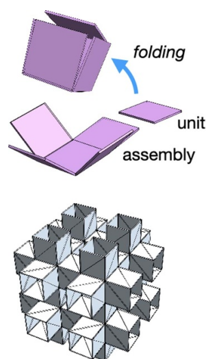
Figure 18. Self-assembling tiles to generate complex or actuating structures. (Top) Self-assembly is an alternate pathway to forming complex orikata at the nanoscale. This can produce origami-like structures that cannot be folded from a flat sheet without gluing. (Bottom) A model of a triply-periodic orikata that can be formed with triangular units having the symmetry cubic symmetry. This cannot be folded from a flat sheet of paper but could be assembled from triangular units following simple rules.
