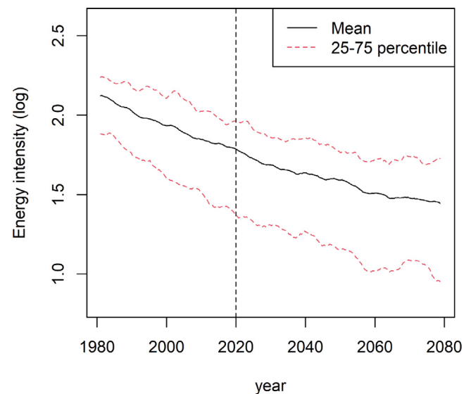
Fig. 2. Energy intensity over time. Logarithmic values. 100 MC runs.
