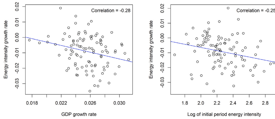
Fig. 3. Correlation between energy intensity growth rate and GDP growth rate (left), initial energy intensity level (right). Correlation stand for the Pearson correlation coefficient. 100 MC runs.
