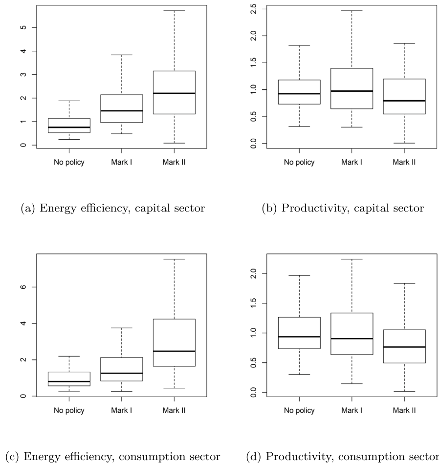
Fig. 5. Boxplots for energy efficiency and productivity in capital and consumption sector in 2080. Data are in terms of no policy scenario mean. 100 MC runs.
