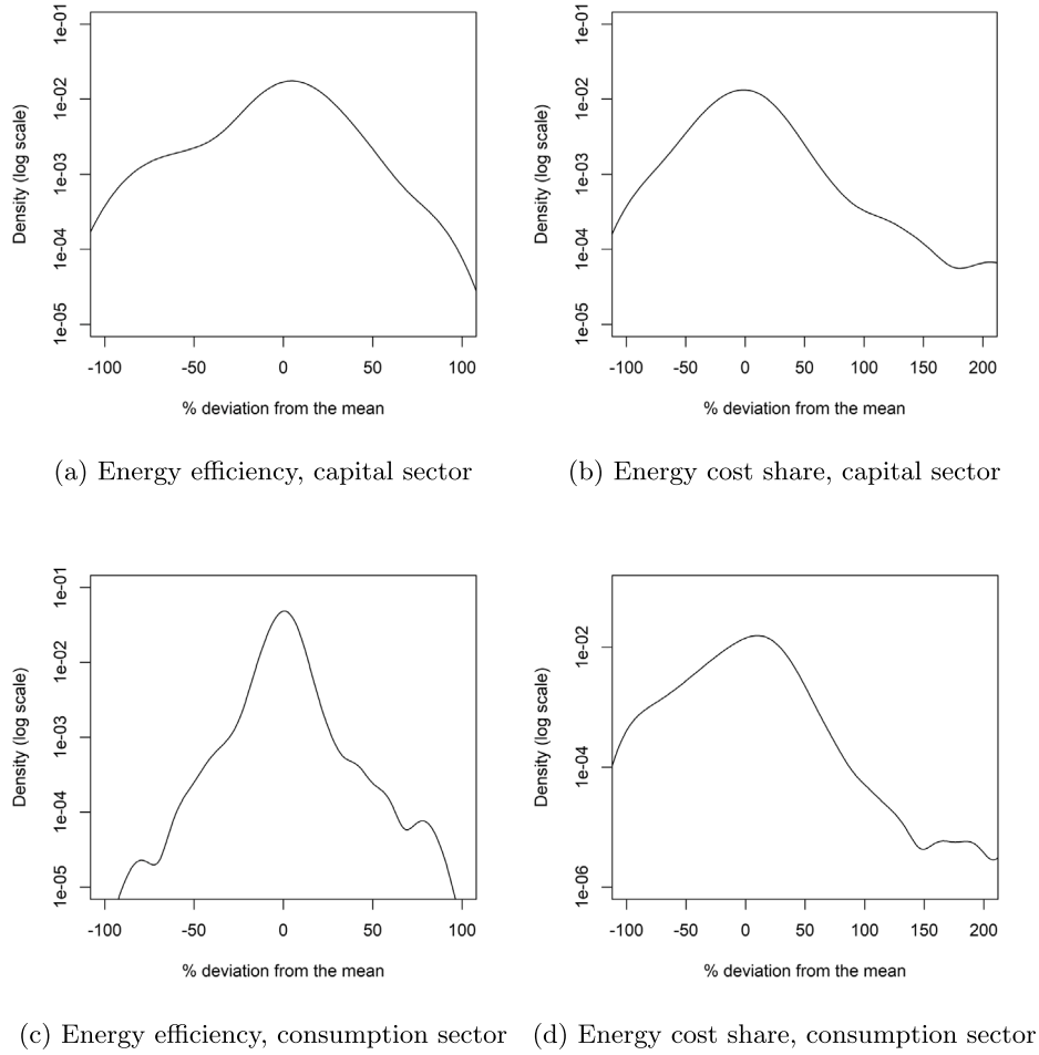
Fig. 4. Energy efficiency and energy cost share heterogeneity across capital-good and consumption-good firms. Kernel distributions.
