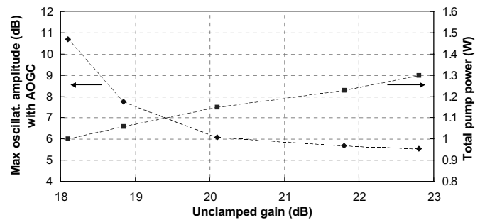
Fig. 7. Maximum amplitude of output probe oscillations at the cascade output (left) and total required pump power (right) versus amplifier unclamped gain in a 18-dB clamped RA.
