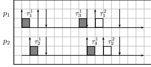
Figure 5: Counterexample for the simple protocol.
