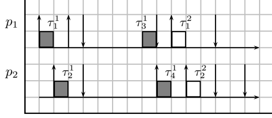
Figure 6: The example of Figure 5 scheduled by DDSP.
