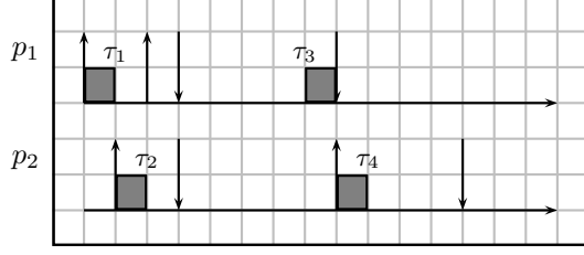
Figure 4: Deadlines assigned by the simple protocol.
