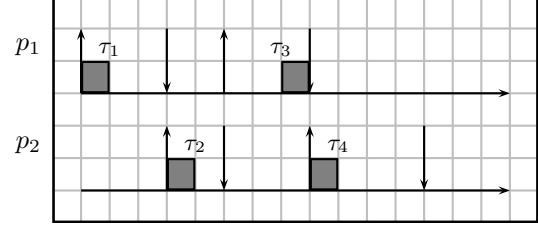
Figure 3: Deadlines assigned by the optimal protocol.
