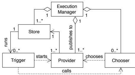
Fig. 3. Simplified UML class diagram of the core components
