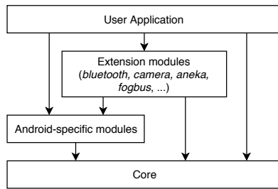
Fig. 2. High-level overview of the library software components
