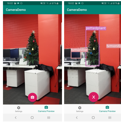
Fig. 5. Object detection demo app: on the left, preview screen; on the right, result screen.
